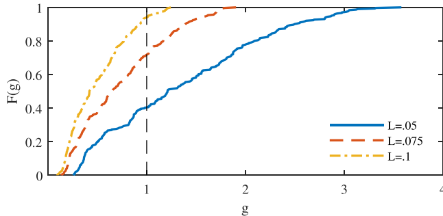
Fig. 12. Empirical cumulative distribution function of global stress rate for RL//C circuit.
