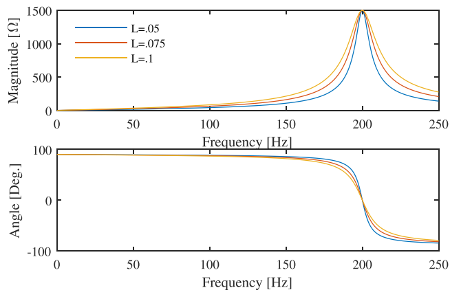
Fig. 8. Frequency response of example RLC circuits.
