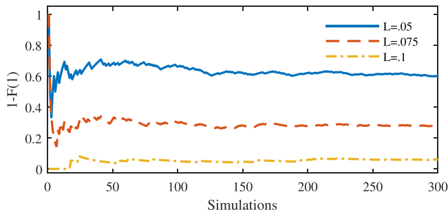
Fig. 11. Convergence of Monte Carlo method for the RL//C circuit.
