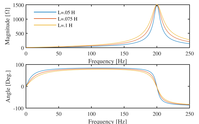
Fig. 6. Frequency response of example RL/c circuits.
