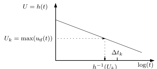
Fig. 3. Example voltage-duration curve.
