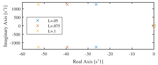
Fig. 9. Pole-zero map of example RLC circuits.
