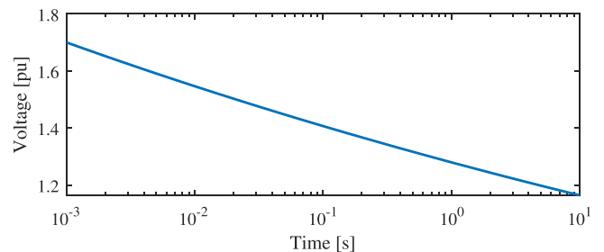
Fig. 10. U-t-curve for case study.
